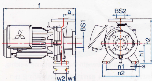
WCM-1505FS, FT / WCM-2205FS, FT / WCM-3705FS, FT
